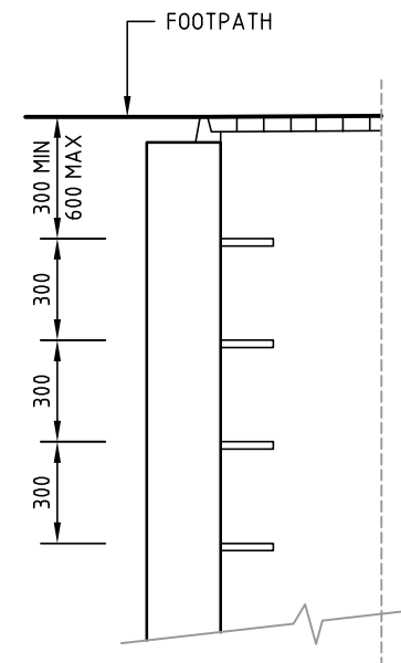
STEP IRON SPACING DETAIL
