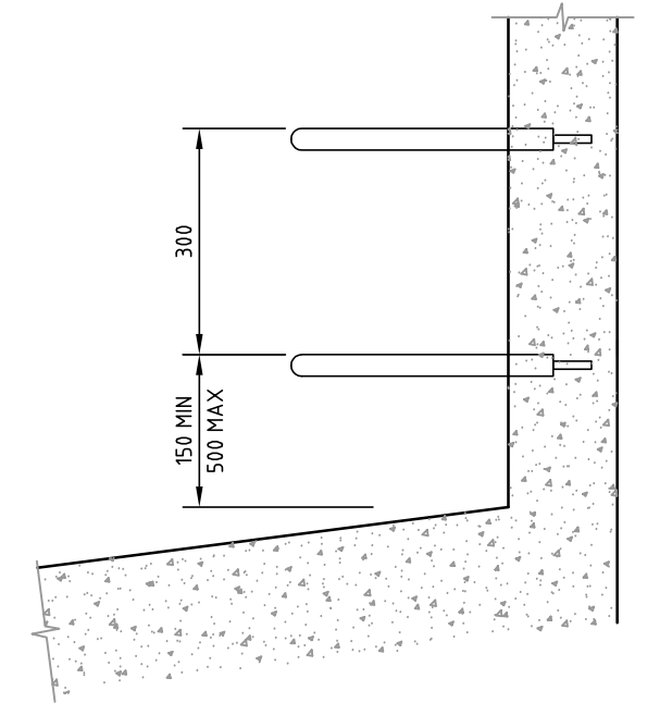
CAST IN-SITU STEP IRONS
