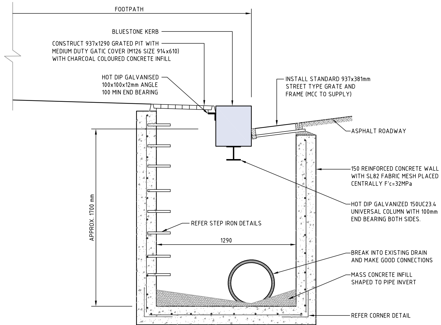
GRATED MANHOLE DRAINAGE PIT
