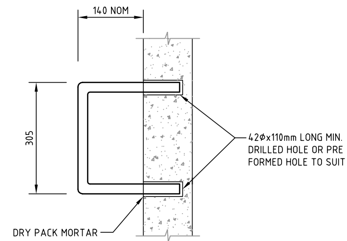
DRILLED OR PRE-FORMED HOLES
