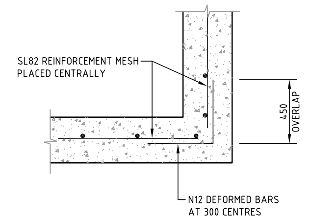
TYPICAL CORNER DETAIL
